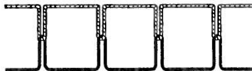
Stitch Type 301
