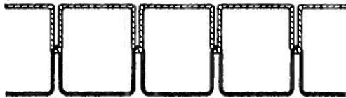
Stitch Type 301
