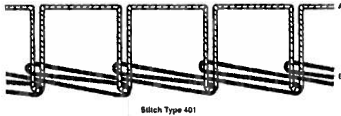
Stitch Type 401
